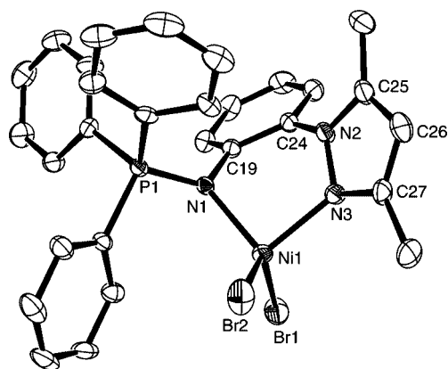
Figure 1. ORTEP drawing of complex 5 (thermal ellipsoids at 30% probability). Selected bond lengths [ \text{\AA} ] and angles [ ^\circ ]: Ni(1)–N(1) 2.002(6) , Ni(1)–N(3) 2.007(6) , Ni(1)–Br(1) 2.3614(13) , Ni(1)–Br(2) 2.3743(13) , P(1)–N(1) 1.624(6) , N(1)–C(19) 1.421(9) , N(2)–N(3) 1.388(8) , N(2)–C(24) 1.434(9) , C(19)–C(24) 1.412(10) ; N(1)–Ni(1)–N(3) 92.2(2) , N(1)–Ni(1)–Br(1) 104.75(17) , N(3)–Ni(1)–Br(1) 108.5(2) , N(1)–Ni(1)–Br(2) 113.81(16) , N(3)–Ni(1)–Br(2) 106.71(18) , Br(1)–Ni(1)–Br(2) 125.71(6) , C(19)–N(1)–Ni(1) 113.3(4) , P(1)–N(1)–Ni(1) 124.4(3) , C(27)–N(3)–Ni(1) 127.4(5) , N(2)–N(3)–Ni(1) 118.3(4) , C(19)–N(1)–P(1) 121.5(5) , N(3)–N(2)–C(24) 119.1(6) .
