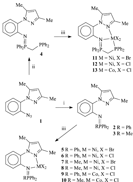
Scheme 2. Synthesis of compounds 2–13 . Reagents and conditions: i) \text{Ph}_2\text{PR} (R = Ph, Me), \text{CH}_2\text{Cl}_2 , room temperature, 12 h; ii) \text{Ph}_2\text{PCH}_2\text{PPh}_2 , \text{CH}_2\text{Cl}_2 , room temperature, 12 h; iii) \text{MX}_2 (M = Ni, X = Br; M = Co, X = Cl) or [\text{NiCl}_2(\text{dme})] , thf, room temperature, 15 h.
