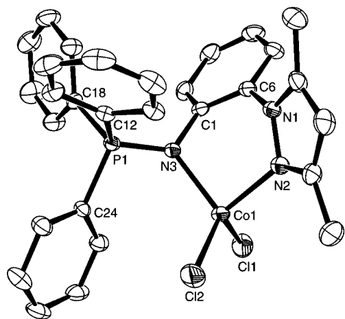
Figure 2. ORTEP drawing of complex 9 (thermal ellipsoids at 30% probability). Selected bond lengths [ \text{\AA} ] and angles [ ^\circ ]: Co(1)–N(2) 2.052(10) , Co(1)–N(3) 2.038(2) , Co(1)–Cl(1) 2.2376(10) , Co(1)–Cl(2) 2.2476(10) , P(1)–N(3) 1.610(2) , N(1)–N(2) 1.385(3) , N(1)–C(6) 1.435(4) , C(1)–C(6) 1.401(4) , N(3)–C(1) 1.427(3) ; N(3)–Co(1)–N(2) 91.54(9) , N(3)–Co(1)–Cl(1) 108.60(7) , N(2)–Co(1)–Cl(1) 113.27(8) , N(3)–Co(1)–Cl(2) 115.95(7) , N(2)–Co(1)–Cl(2) 107.75(8) , Cl(1)–Co(1)–Cl(2) 117.01(4) , N(1)–N(2)–Co(1) 117.84(18) , C(1)–N(3)–Co(1) 111.62(17) , N(2)–N(1)–C(6) 119.4(2) , C(1)–N(3)–P(1) 122.10(18) , C(1)–N(3)–Co(1) 111.62(17) , P(1)–N(3)–Co(1) 125.55(13) .
