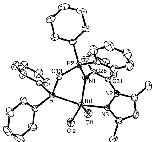
Figure 3. ORTEP drawing of complex 12 (thermal ellipsoids at 30% probability). Selected bond lengths [Å] and angles [°]: Ni(1)–N(1) 2.066(3), Ni(1)–N(3) 2.060(3), Ni(1)–Cl(2) 2.3012(11), Ni(1)–Cl(1) 2.3187(11), Ni(1)–P(1) 2.4001(11), P(2)–N(1) 1.603(3), P(1)–C(13) 1.842(3), P(2)–C(13) 1.806(3), N(2)–N(3) 1.377(4), N(2)–C(31) 1.424(5), N(1)–C(26) 1.405(4), C(26)–C(31) 1.412(5); N(1)–Ni(1)–N(3) 87.00(11), N(1)–Ni(1)–Cl(2) 129.22(9), N(3)–Ni(1)–Cl(2) 92.76(9), N(1)–Ni(1)–Cl(1) 102.94(9), N(3)–Ni(1)–Cl(1) 94.35(9), Cl(2)–Ni(1)–Cl(1) 127.65(5), N(1)–Ni(1)–P(1) 80.64(8), N(3)–Ni(1)–P(1) 167.57(9), Cl(2)–Ni(1)–P(1) 96.05(4), Cl(1)–Ni(1)–P(1) 87.20(4), P(2)–N(1)–Ni(1) 118.82(15), C(26)–N(1)–Ni(1) 114.9(2), C(26)–N(1)–P(2) 126.2(2), N(2)–N(3)–Ni(1) 122.8(2), C(13)–P(1)–Ni(1) 99.02(12), N(1)–P(2)–C(13) 106.93(15).
